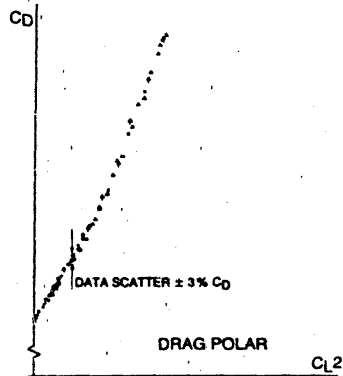
FIG. 14: Repeatability of Flight Test Data
