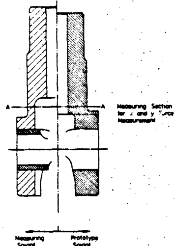
Fig. 10 COMPARISON BETWEEN MEASURING SPIGOT AND PROTOTYP SPIGOT
