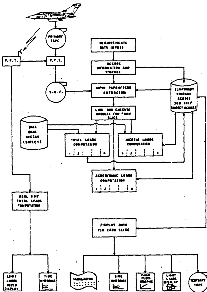
Fig. 18 FLIGHT TEST DATA PROCESSING
