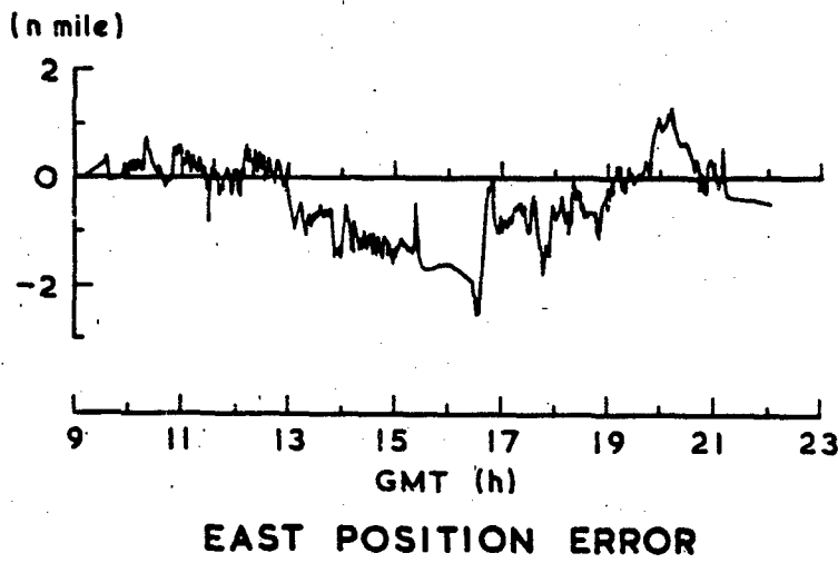
TYPICAL OMEGA POSITION ERRORS
