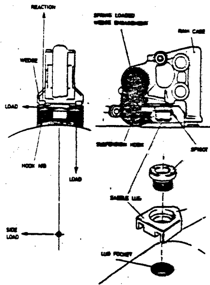
Fig. 4 PRINCIPLE OF MKC SYSTEM
