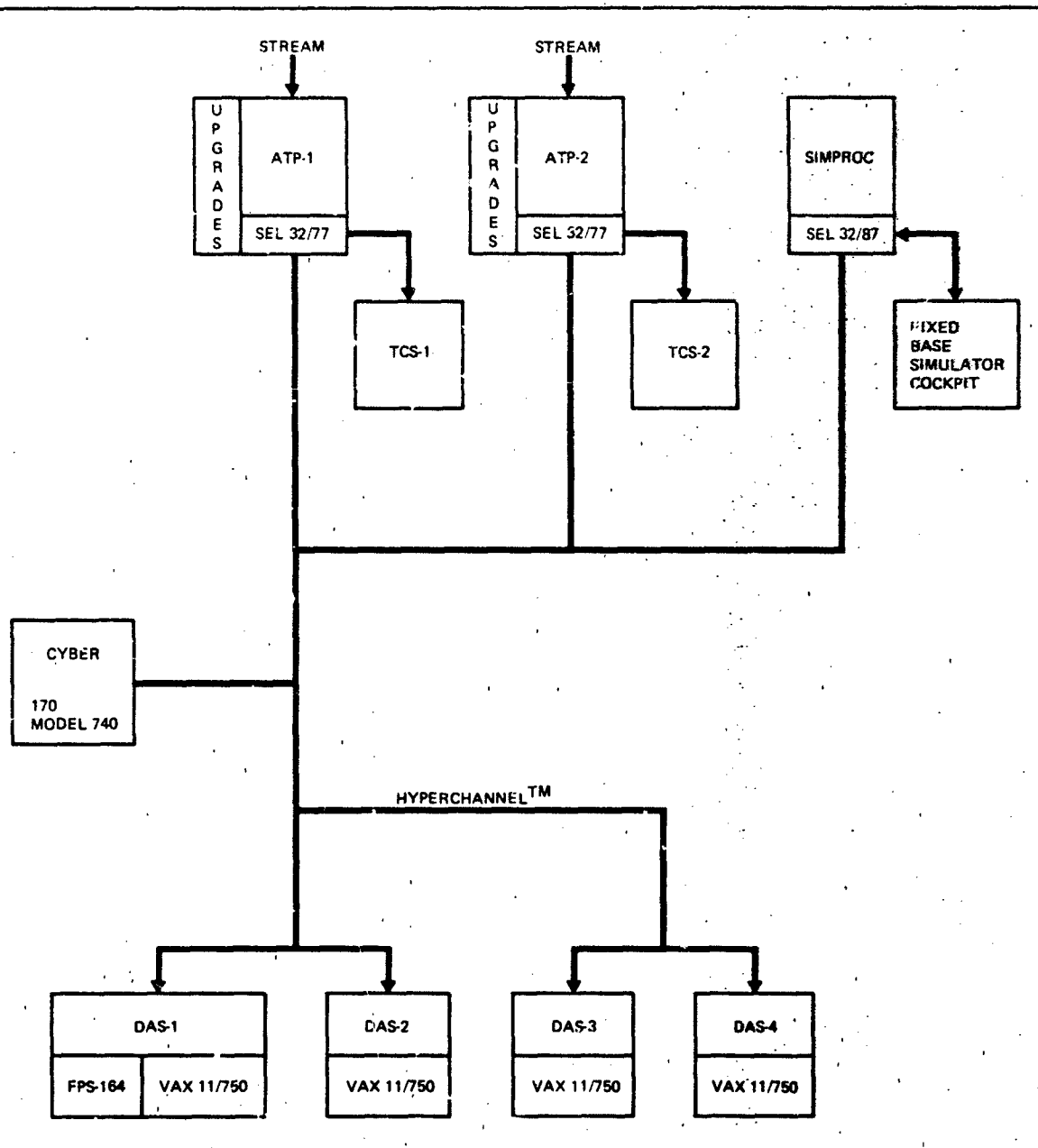
Fig. 3 NDCS Baseline Configuration
