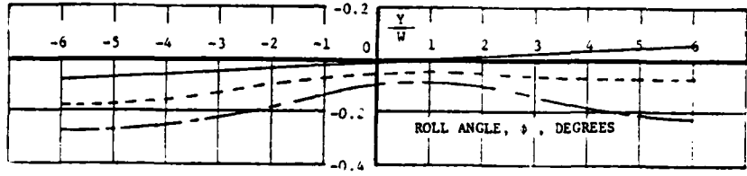
FIGURE A-2.3(g). SIDE FORCE V. ROLL AND YAW ANGLE, \theta = 1^\circ .
