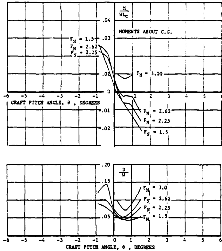
FIGURE A-2.2(d). PITCH MOMENT AND DRAG V. PITCH ANGLE AND FROUDE NO.
