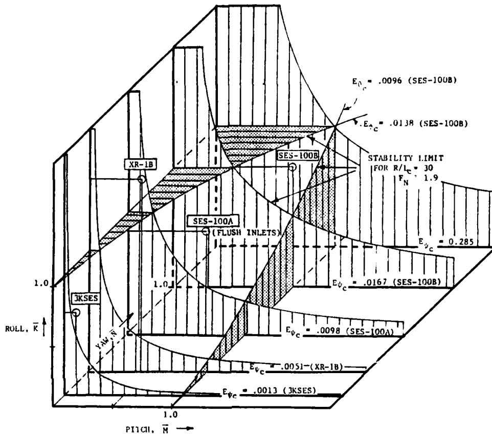
FIGURE 3-28. LIMITS OF SES PITCH, ROLL AND YAW STABILITY IN COMPARISON WITH STABILITY CHARACTERISTICS OF DIFFERENT SES ( F_N \approx 1.9 , R/L_c = 30 ).
