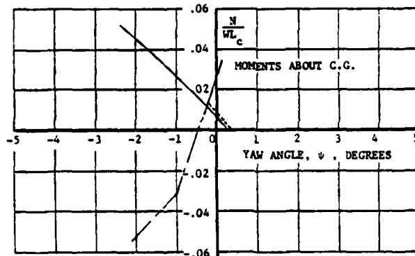
FIGURE A-2.2(g). YAW MOMENT V. YAW ANGLE AND PITCH ANGLE @ F_N = 2.06 (PODS).
