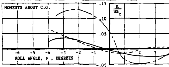
FIGURE A-2.3(bb). ROLL MOMENT V. ROLL AND YAW ANGLE, \theta = -0.5^\circ ; F_N = 3.04 .
