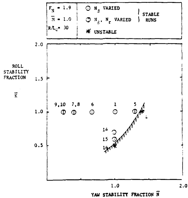
FIGURE 3-21. EFFECT OF VARIATION OF ROLL AND YAW STABILITY ON SIMULATED SES-100B RUDDER REVERSAL MANEUVERS AT CONSTANT TURN RADIUS ( R/L_c=30 ) AND SPEED (50 KNOTS, F_N=1.9 ).
