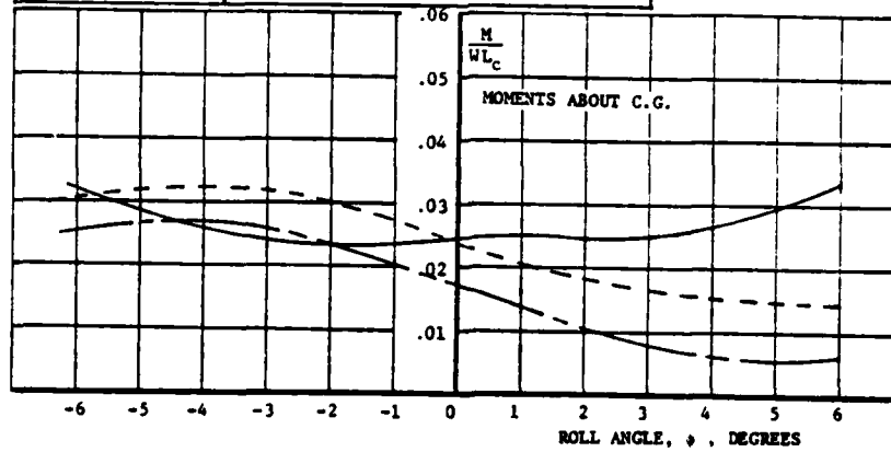
FIGURE A-2.3(f). PITCH MOMENT V. ROLL AND YAW ANGLE, \theta = -1^\circ .
