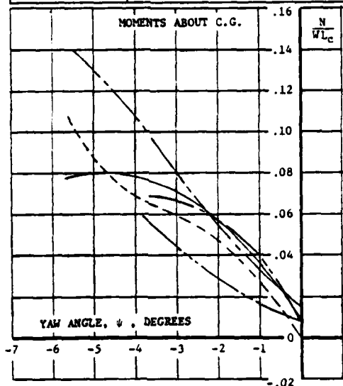
FIGURE A-2.3(k). YAW MOMENT V. YAW AND ROLL ANGLE, \theta = +1.5^\circ .
