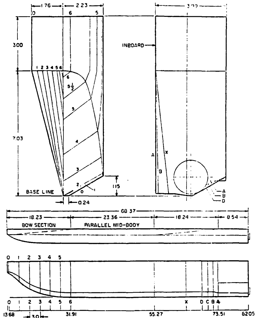
FIGURE 3-4. LINE PLAN OF SES-100B SIDEWALL. (SIT JUN 74)
