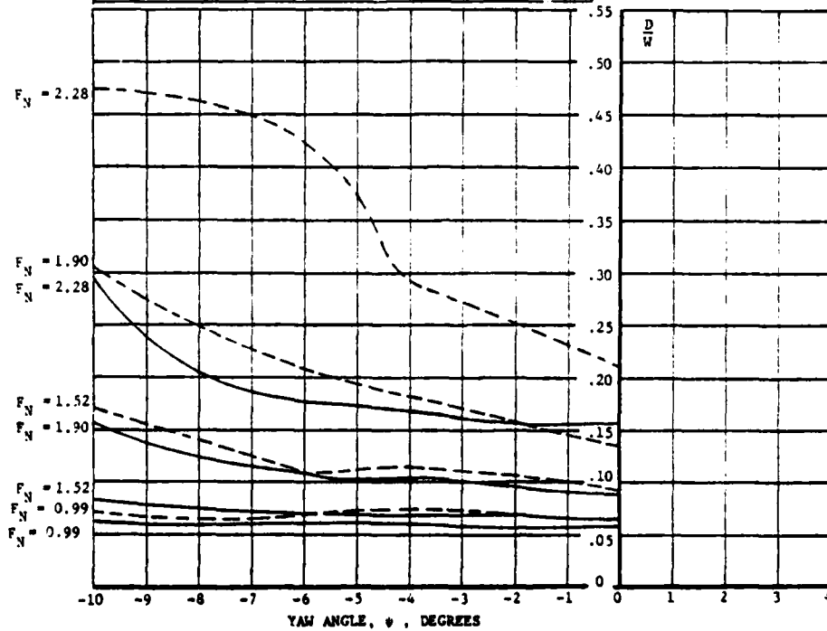
FIGURE A-2.1(d). DRAG V. YAW AND PITCH ANGLE AND FROUDE NO.
