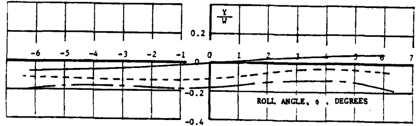
FIGURE A-2.3(h). SIDE FORCE V. ROLL AND YAW ANGLE, \theta = -1^\circ .
