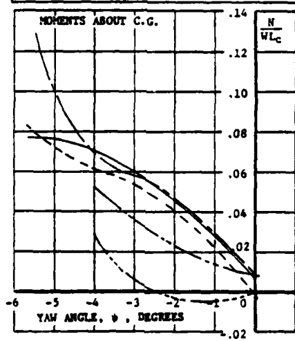
FIGURE A-2.3(l). YAW MOMENT V. YAW AND ROLL ANGLE, \theta = +1.5^\circ .
