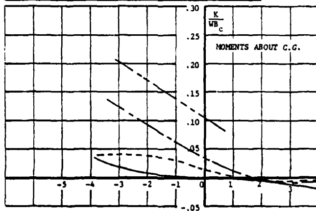
FIGURE A-2.3(x). ROLL MOMENT V. ROLL AND YAW ANGLE, \theta = -1.5^\circ ; F_N = 2.47 .
