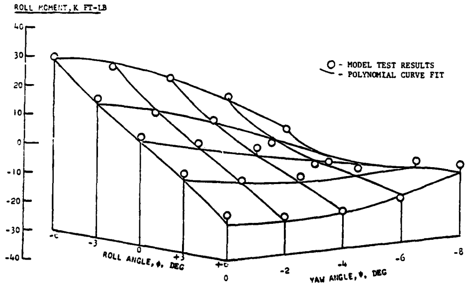
FIGURE 3-8. COMPARISON OF SES-100B MODEL ROLL MOMENT DATA WITH CURVE FIT. TRIM = 1 DEG, SPEED = 18.2 FPS (SIT JUN 74)
