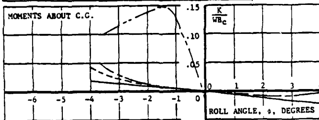
FIGURE A-2.3(w). ROLL MOMENT V. ROLL AND YAW ANGLE, \theta = -0.5^\circ ; F_N = 2.47 .
