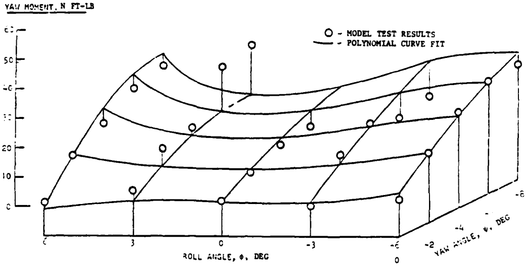
FIGURE 3-7. COMPARISON OF SES-100B MODEL YAW MOMENT DATA WITH CURVE FIT. TRIM = 1 DEG, SPEED = 18.2 FPS (SIT JUN 74)
