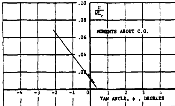
FIGURE A-2.2(h). YAW MOMENT V. YAW ANGLE AND PITCH ANGLE @ F_N = 2.62 (PODS).
