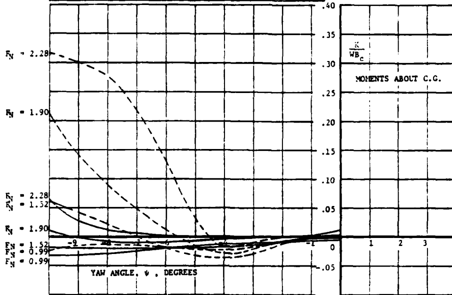
FIGURE A-2.1(i). ROLL MOMENT V. YAW AND PITCH ANGLE AND FROUDE NO.
