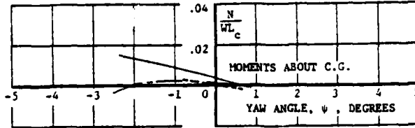
FIGURE A-2.2(f). YAW MOMENT V. YAW ANGLE AND PITCH ANGLE @ F_N = 1.50 (PODS).
