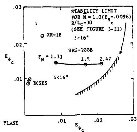
FIGURE 3-27. COMPARISON OF SES STABILITY CHARACTERISTICS WITH STABILITY LIMITS FOR F_N = 1.9 and R/L_c = 30 .
