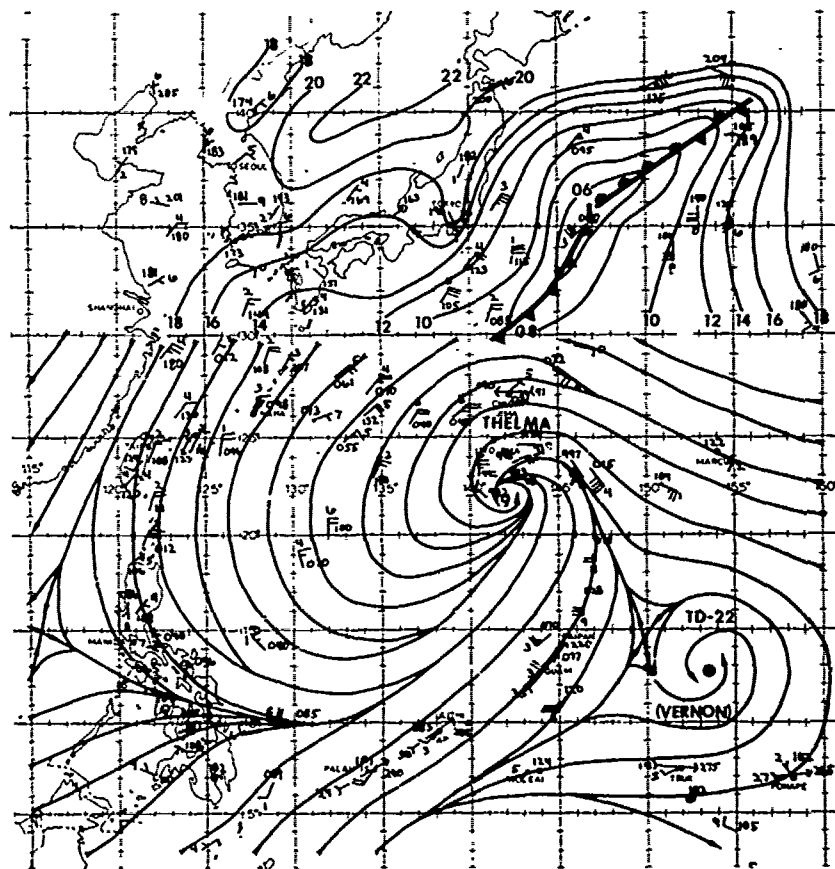
FIGURE 3-22-3. The 280000Z September 1980 surface wind data and streamline analysis. Winds speeds are in knots.
