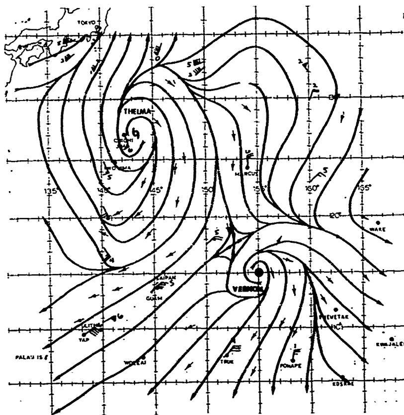
FIGURE 3-22-1. Upper-level streamline analysis (near the 200 mb level; at 290000Z September 1980. Data are rawinsonde and aircraft winds (→⊙) and satellite-derived wind vectors (→). Winds are in knots.
