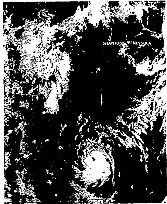
FIGURE 3-07-1. Tropical Storm Herbert at 45 kt (23 m/sec) intensity making landfall over southern China, 28 June 1980, 0316Z. (DMSPI imagery)
