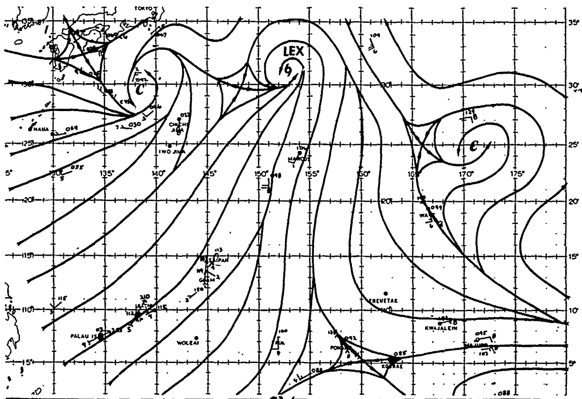
FIGURE 3-13-1. The 051200Z August 1980 surface 1/gradient-level (ddd←66) wind data and streamline analysis. Wind speeds are in knots.
