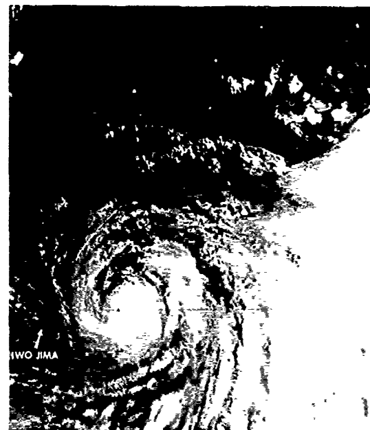
FIGURE 3-12-2. Typhoon Lex at maximum intensity of 80 kt (41 m/sec), 2 August 1980, 2242Z. Iwo Jima is about 155 nm (285 km) west of Lex. (NOAA6 imagery)
