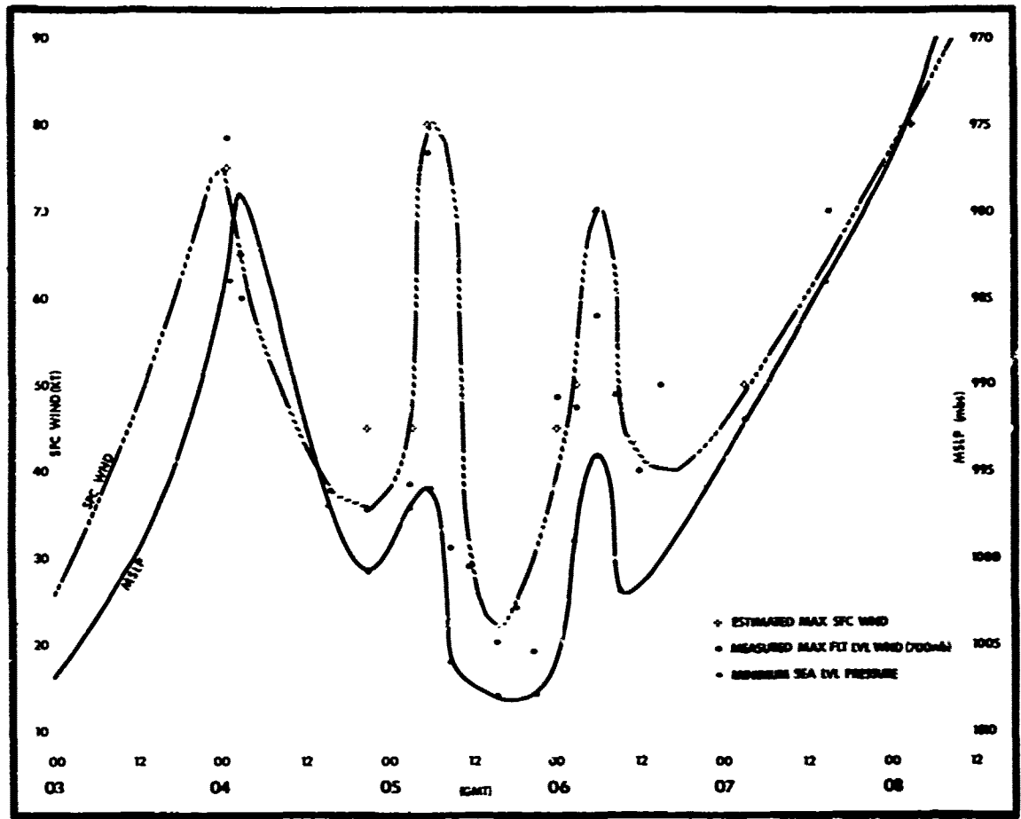
FIGURE 3-23-3. Smoothed traces of Myone's maximum wind speed and minimum sea level pressure versus time for the period 3-9 October 1989.
