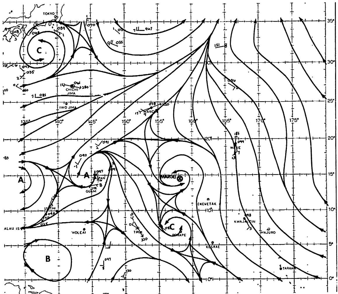
FIGURE 3-13-3. The 071200Z August 1980 surface (—) / gradient-level (ddd ← cff) wind data and streamline analysis. Wind speeds are in knots.
