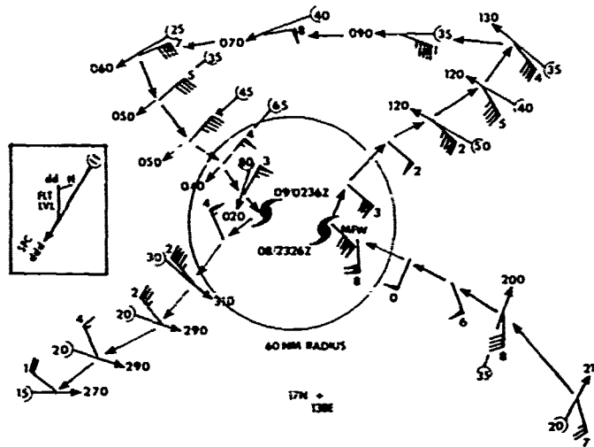
FIGURE 3-23-2. Plot of aircraft reconnaissance data for the 082326Z and 090236Z October 1986 fixes of Typhoon Wynne.
