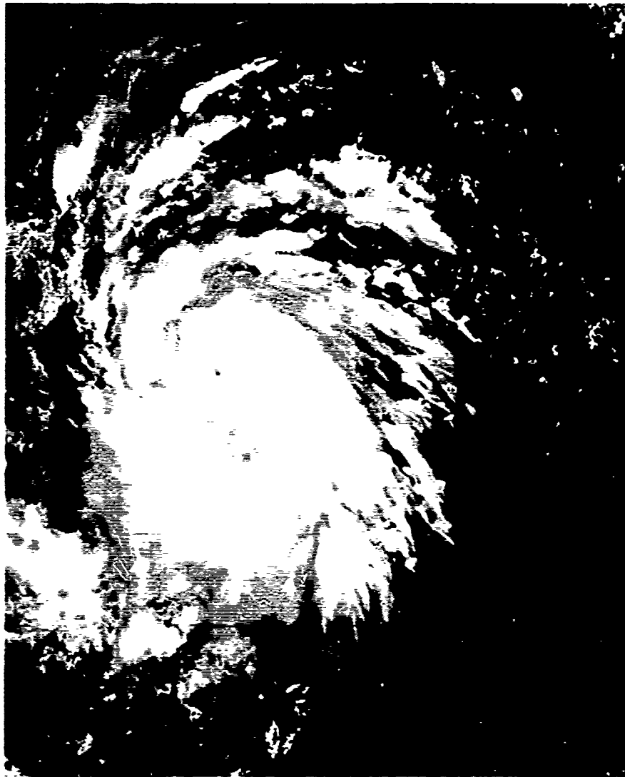
FIGURE 3-11-2. Typhoon Kim at approximately 110 kt (57 m/sec) intensity before she reached super typhoon strength, 24 July 1980, 0125Z. (DMSF imagery)
