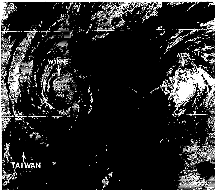
FIGURE 3-24-1. Visual imagery of Tropical Storm Alex at 30 kt (15 m/sec) intensity, 12 October 1980, 2314Z. (NOAA6 imagery)
