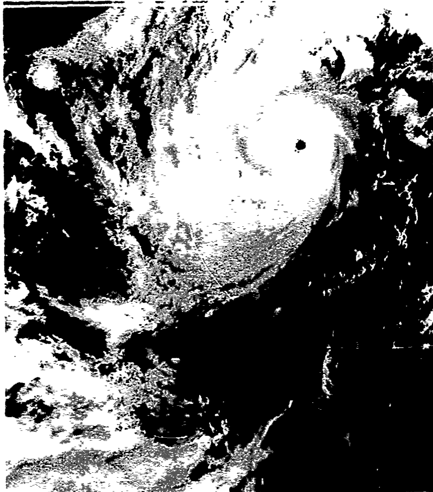
FIGURE 3-19-3. Typhoon Percy with 110 kt (57 m/sec) maximum surface winds while intensifying rapidly to near super typhoon strength, 17 September 1980, 0645Z. (Tiroc 4 imagery)
