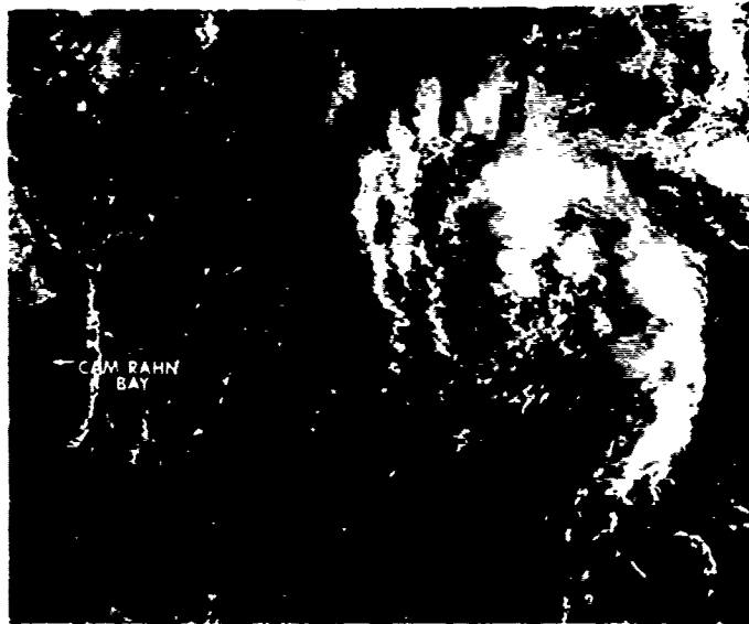
FIGURE 3-01-3. The remnant of TD 01 in the South China Sea showing signs of regeneration, 26 March 1980, 0206Z. (DMS imagery)
