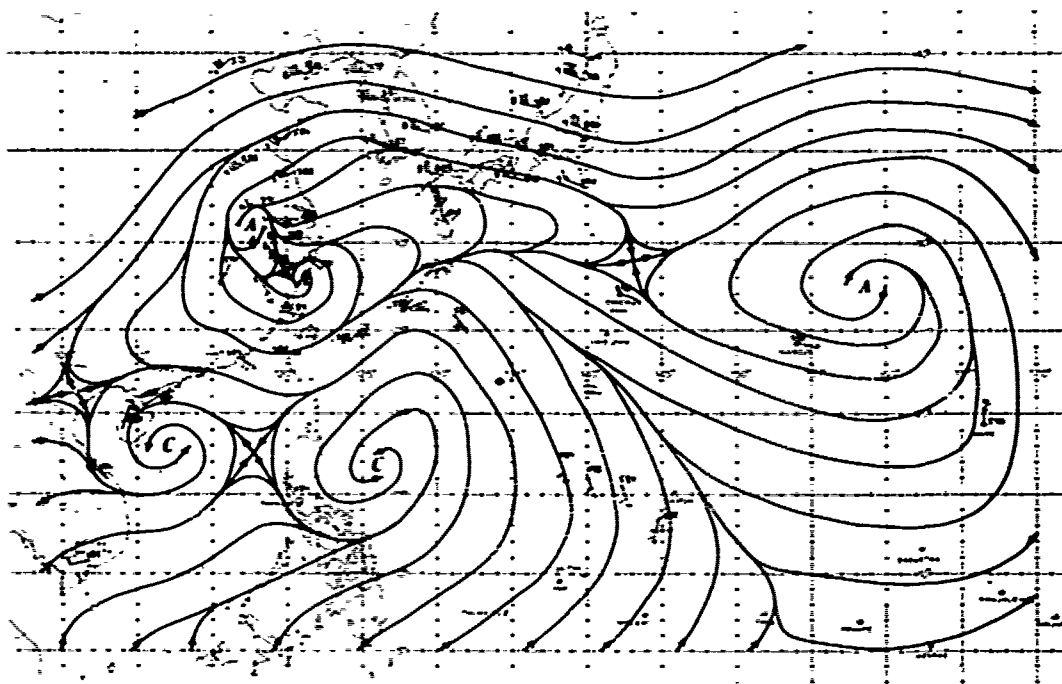
FIGURE 3-20-1. The 141200Z September 1950 500 mb streamlines analysis. Wind speeds are in knots.
