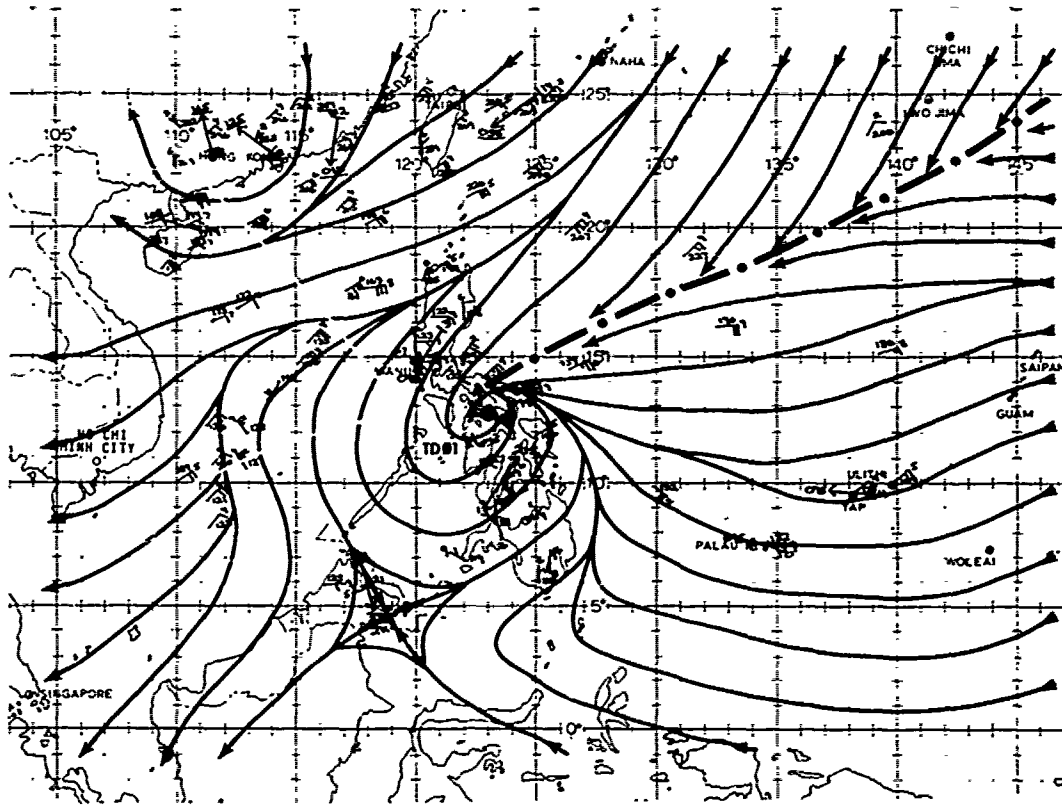
FIGURE 3-01-2. The 240000Z March 1980 surface (---) /gradient-level (ddd---) wind data and streamline analysis. Wind speeds are in knots.
