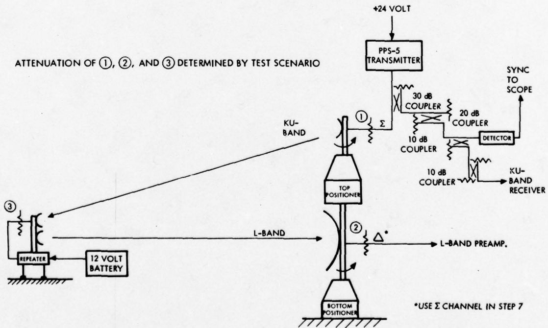
Figure 3-21. System Connection for Repeater Interrogation
