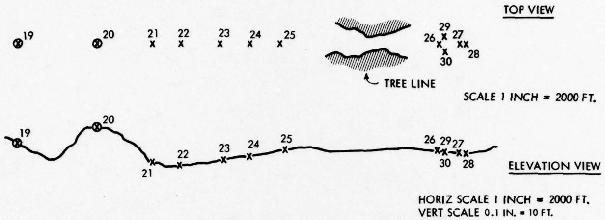
Figure 3-20. Foliage/Terrain Obstruction Effects Test Geometry
