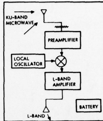
REPEATER
