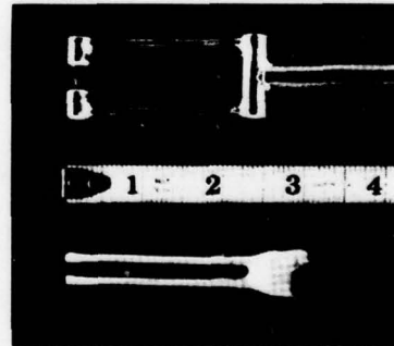
3b. The Iowa Sediment Concentration Measuring System (ISCMS). Electro-optical probes used to detect temporal changes in suspended sediment in the laboratory (From Locher, et al. , 1977; Fig. 2).
