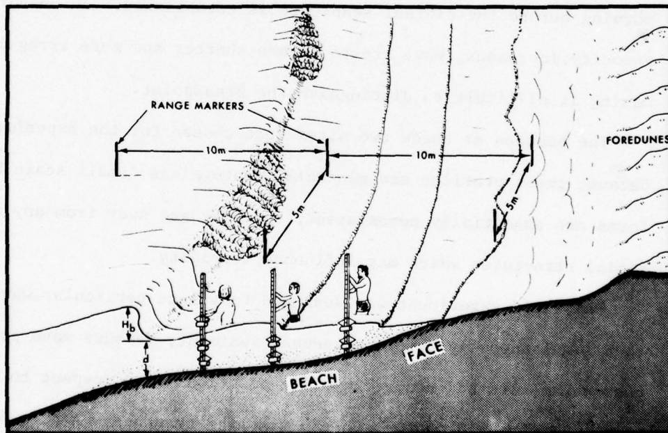
Figure 18. Sketch of the sampling arrangement showing samplers in place. Operators stood down-drift from sample point holding apparatus above bed until sampling instant. Range markers provided reference marks to locate sampling positions, measure longshore current velocity and distances from the breakpoint.
