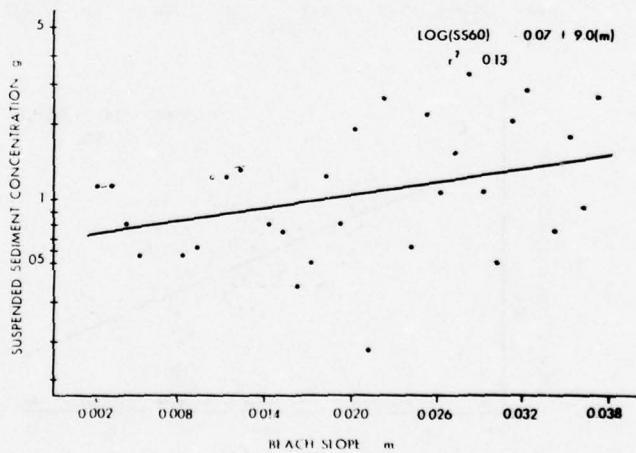
Figure 37. Mean SS10 (a), SS30 (b) and SS60 (c) vs. beach slope (m) showing general increase in concentration with increasing slope. Indicated regression lines account for up to 31% of the variability in mean concentration.
