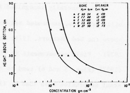
Figure 6. Distribution of suspended sediment at 10, 60 and 90 cm above the bed measured using the in situ bulk water sampler shown in Fig. 13c (From Inman, 1977).
