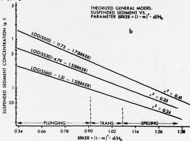
Figure 49(a and b). General linear models for the distribution of suspended sediment concentration in the breaker zone, based on the present experiment. (a) Ratio d_b/H_b by sample position and (b) Parameter BRKER by sample position.
