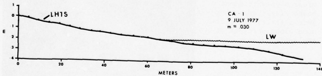
Figure 16. Profiles at station CA1 on 14 June and 9 July 1977, showing a generally featureless profile. Small amplitude ripples or bed forms are essentially absent at both stations.
