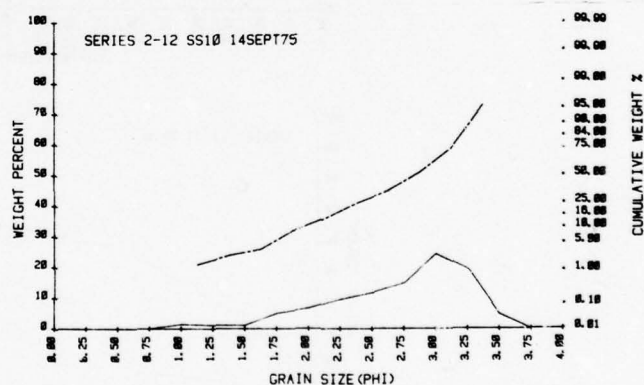
Figure 45. Grain size frequency curves for an array of suspended sediment samples and corresponding bed sample. From top to bottom, size distribution for SS60, SS30, SS10 and the bed. Note wide range of sizes on the bed at this location. The label +100-1 in (d) refers to distance in meters from a benchmark on land. The range of sizes and mean size decreases for suspended samples going up in the water column.
