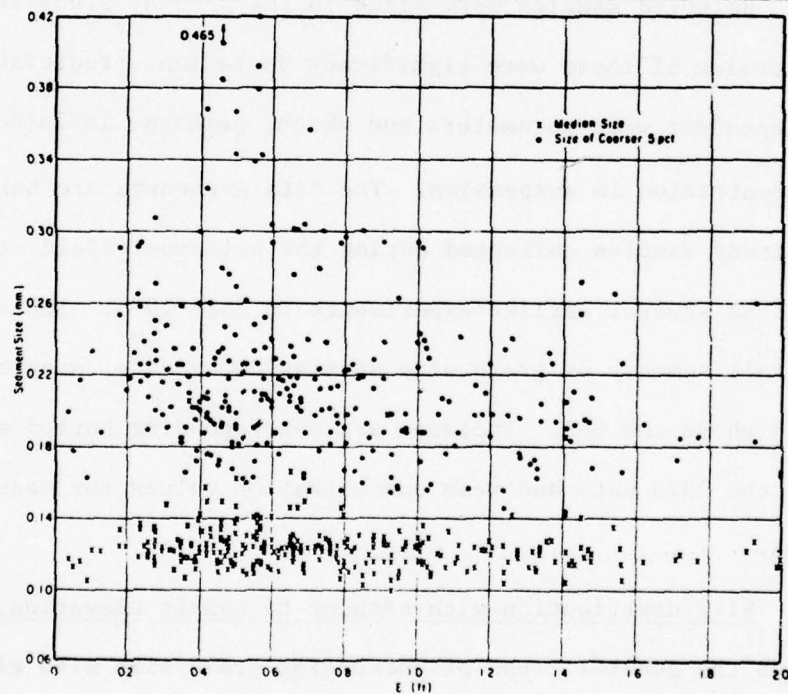
Figure 43. Median (x's) and coarse (dots) suspended sediment sizes by nozzle elevation above the bed (E) for time-averaged pump samples. Note general increase in size of the coarsest fraction near the bed. (From Fairchild, 1977; Fig. 11).
