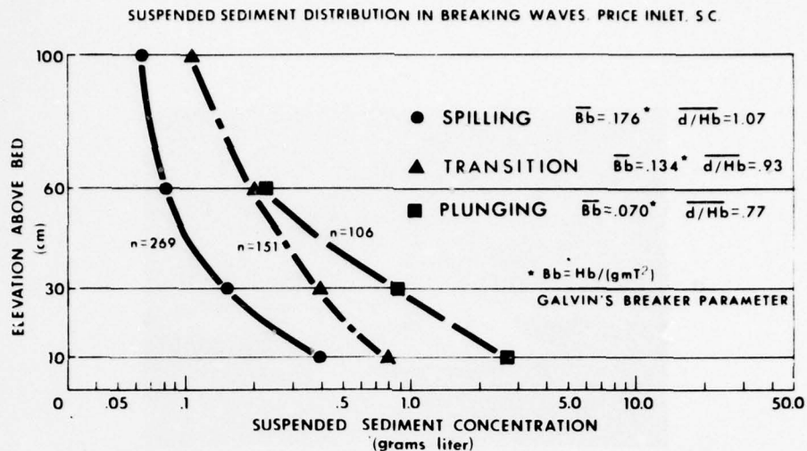
Figure 31. Suspended sediment distribution in the outer surf zone between 1 and 10 m landward of the breakpoint. Mean concentrations are plotted by elevation above the bed for spilling and plunging type breakers. An intermediate wave type, referred to as transition, exhibiting characteristics of spilling and plunging waves is also plotted (triangles).
