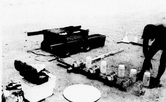
Figure 22a. Array of 5 samples ready for transfer to 2 l. Nalgene holding jars. Sampler bottles are calibrated to measure volume collected.
