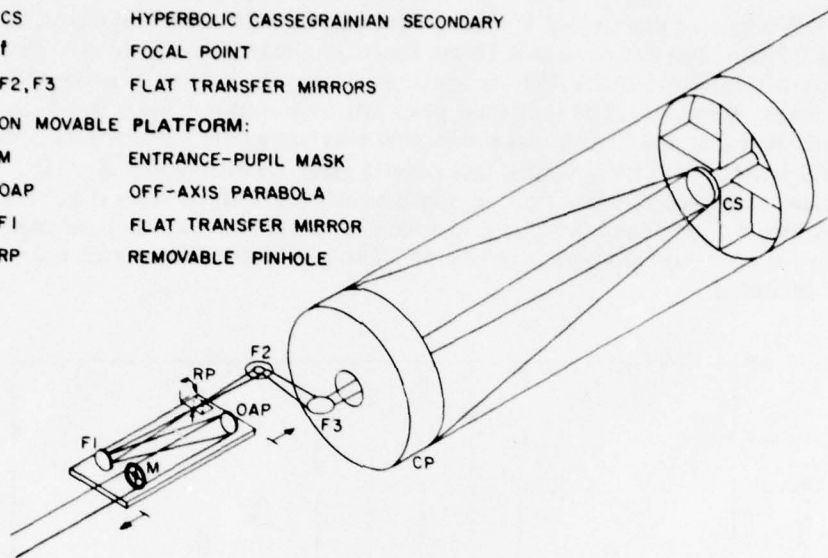
Fig. 3 - Cassegrainian telescope
