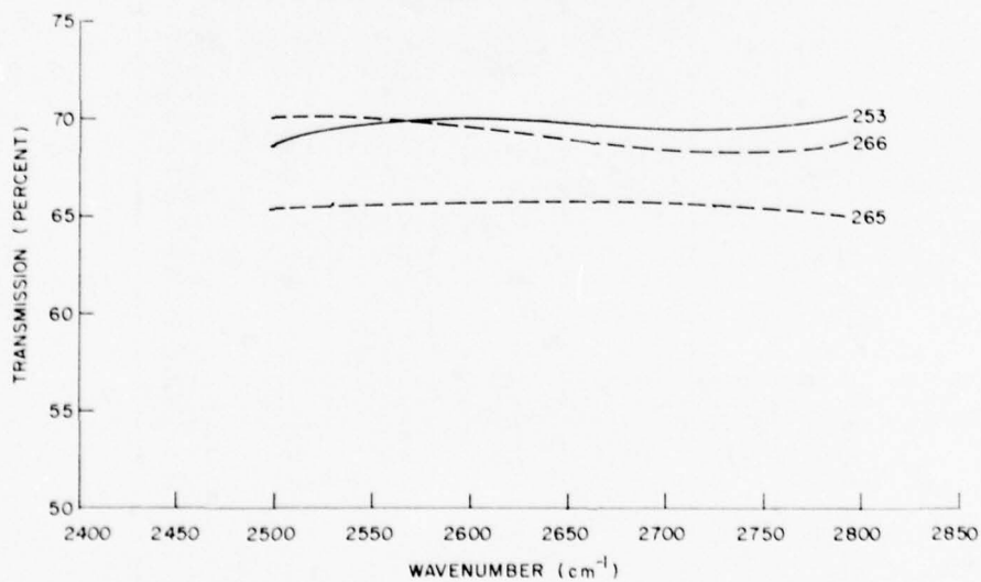
Fig. 13 - Zero-path transmissions vs wavenumber for the second test series
