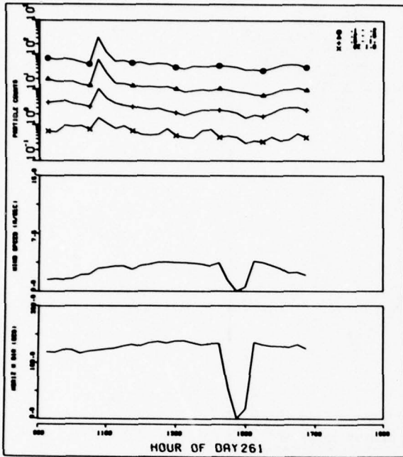
Fig. 28e — Particle counts, wind speed, and horizontal wind direction vs time
