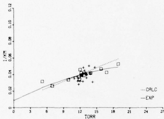
Fig. 30o — Molecular absorption vs water-vapor pressure, P 19 DF laser line
