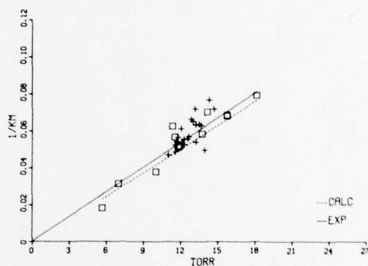
Fig. 30p — Molecular absorption vs water-vapor pressure, P 25 DF laser line
