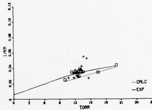
Fig. 30h — Molecular absorption vs water-vapor pressure, P 36 DF laser line
