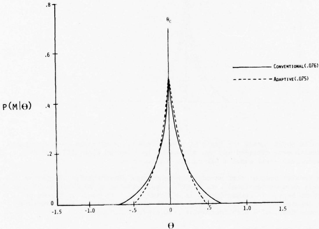
Figure 18 shows P(M|\theta) curves for the same strategies with item discriminations of \alpha=2.0 . The same general results were obtained, except that the differences
