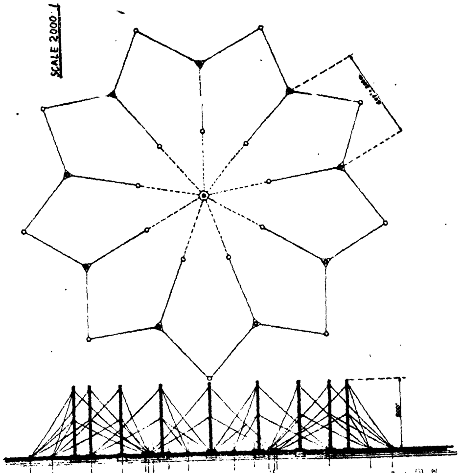
FIG. 5 - ALTERNATE PRELIMINARY PROPOSAL OF OMEGA FERRITE ANTENNA
