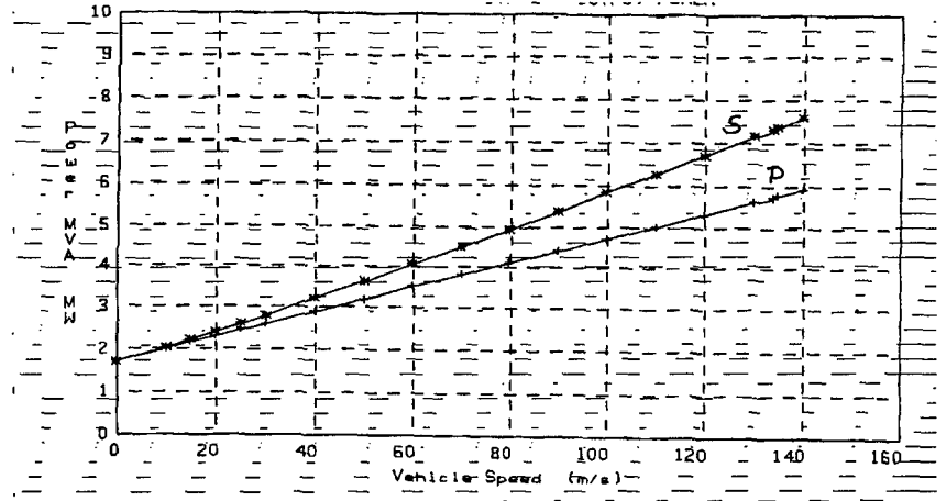
GR 2 CAR-CONSIST(A1): TABLE III. Electrical Performance-Converter Station Output
