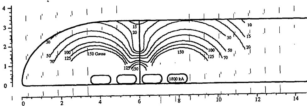
Figure 70. Top view of stray fields for Foster-Miller aiding-flux arrangement.
