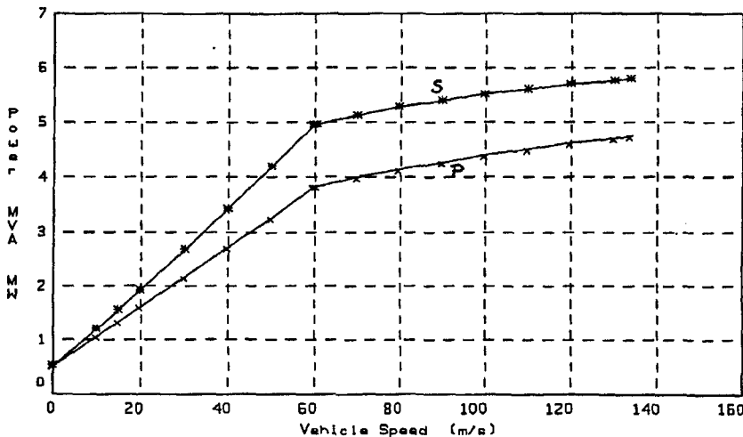
TR07 2 CAR-CONSIST: TABLE II. LSM Electrical Performance at LSM Block
