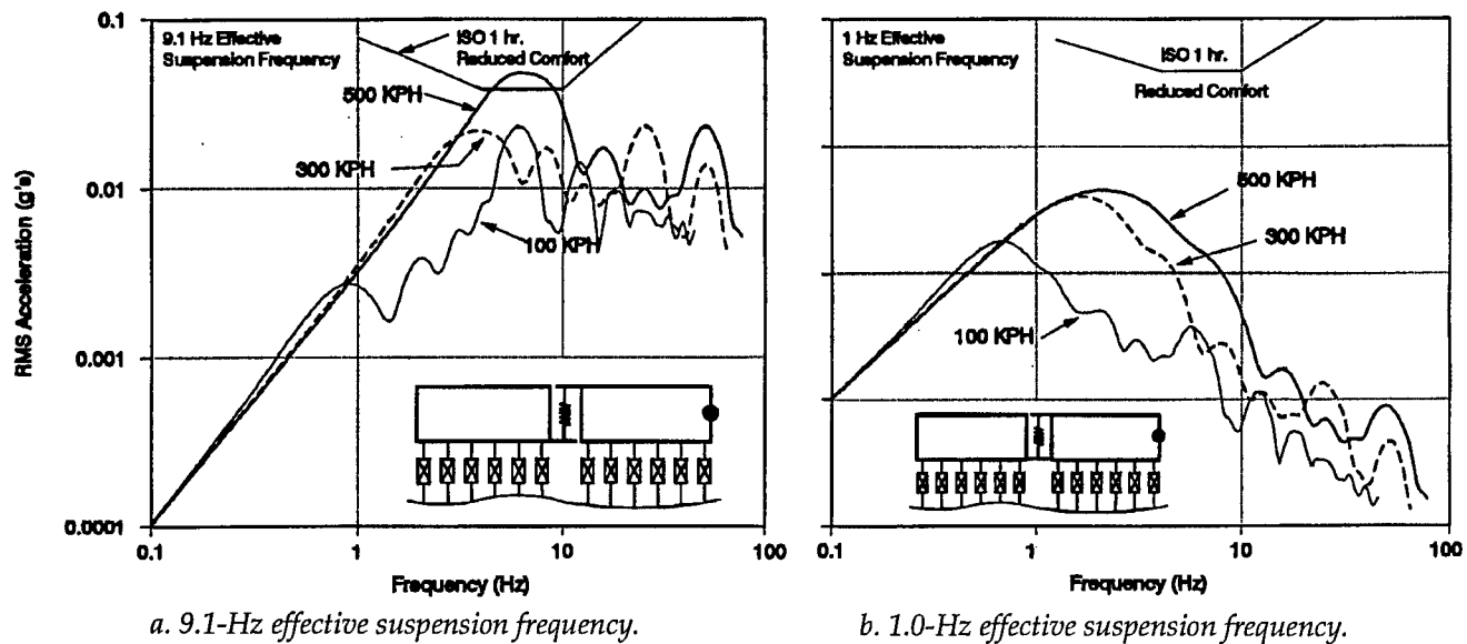
Figure 101. Grumman vehicle response to random roughness (rigid guideway).
