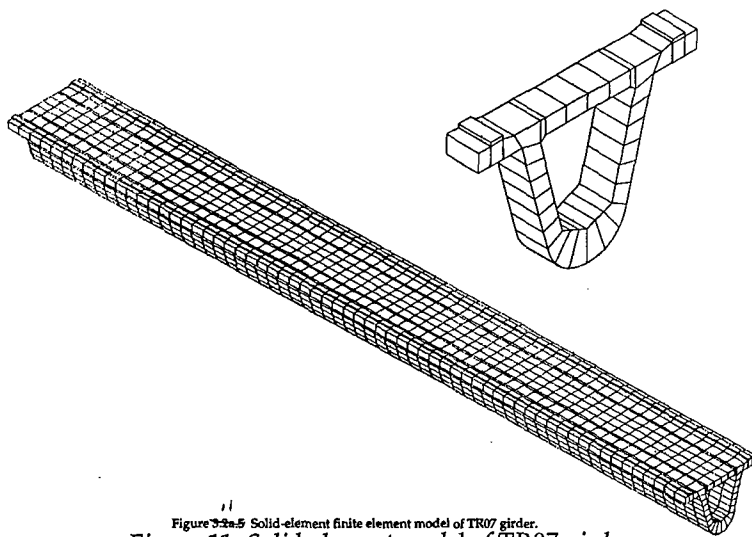
Figure 11. Solid-element model of TR07 girder.
