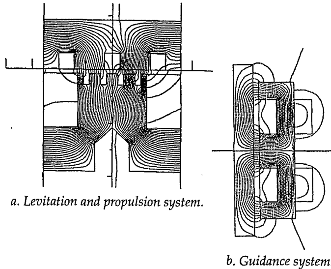
Figure 53. TR07 flux patterns.
