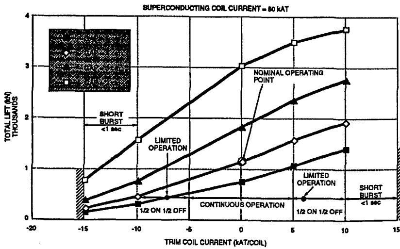
Figure 77. Total normal force vs. trim current for Grumman suspension.
