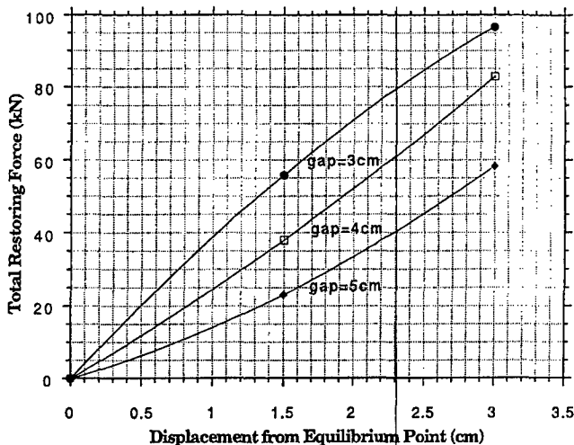
Figure 80. Grumman restoring force for constant current for one magnet moved parallel to rail face ( I = 50 \text{ kA} ).
