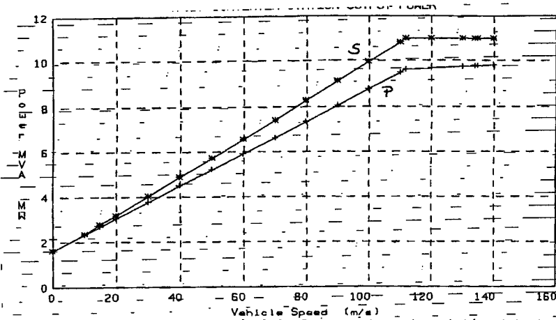
BECHTEL-CM: TABLE III: Electrical Performance-Converter Station Output
