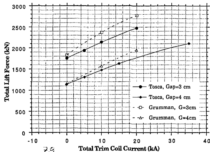
Figure 78. Comparison between ANL and Grumman computations of lift forces (with trim coil as variable; I_{sc} = 50 kA).
