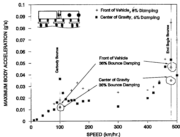
Figure 95. Foster-Miller maximum carbody acceleration vs. speed. Center of gravity and front of vehicle vertical acceleration on a flexible guideway.
