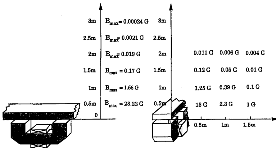
Figure 81. Stray fields around the center of Grumman magnet ( I = 50 \text{ kA} ; g = 4 \text{ cm} ).
