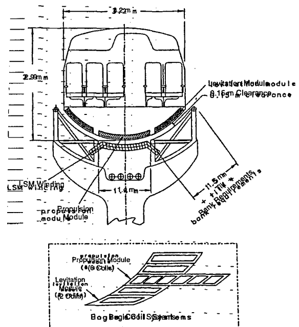
b. Vehicle cross-section and bogie coils.
