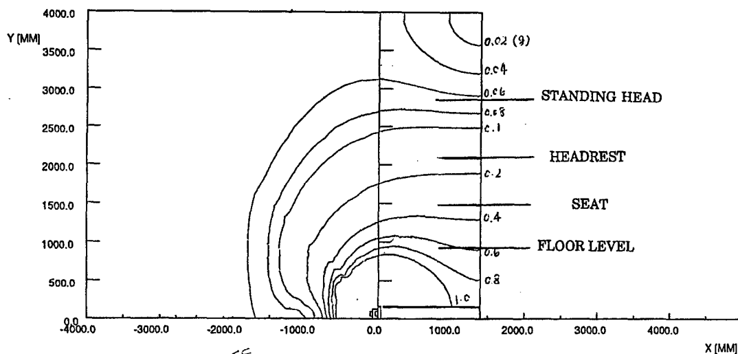
Figure 59. Flux density (G) around TR07 guidance magnet.
