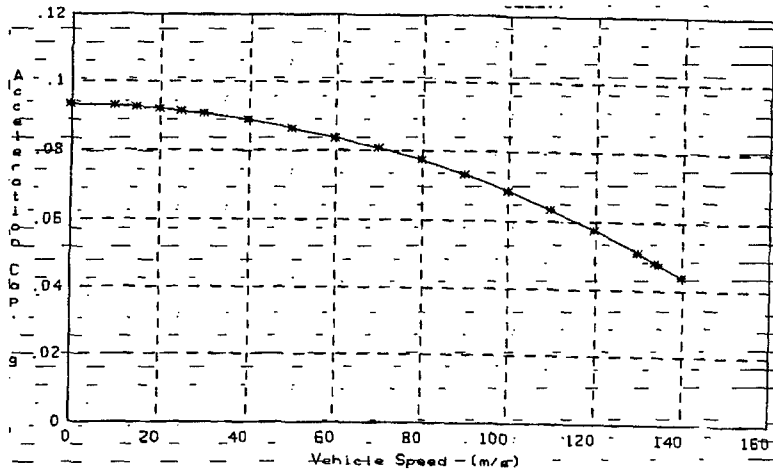
GR 2-CAR-CONSIST(A1): TABLE IV. Acceleration Capability
