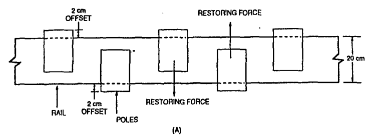
Figure 74 (cont'd). Baseline magnetic structure of the Grumman concept.
