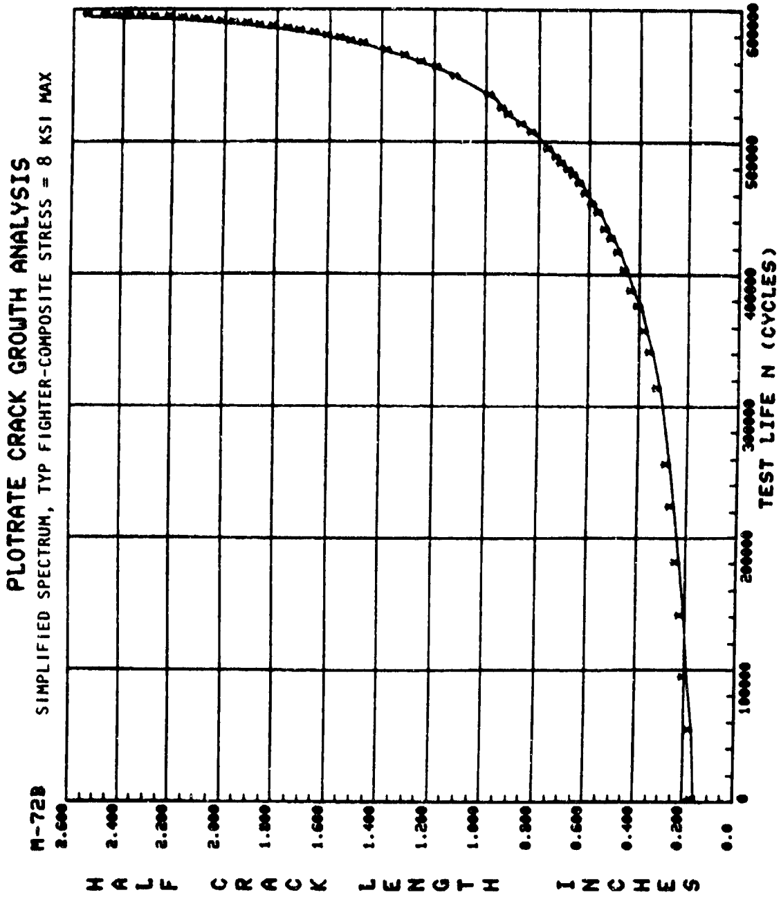
Figure 93. Crack growth curve for test M-72B.
