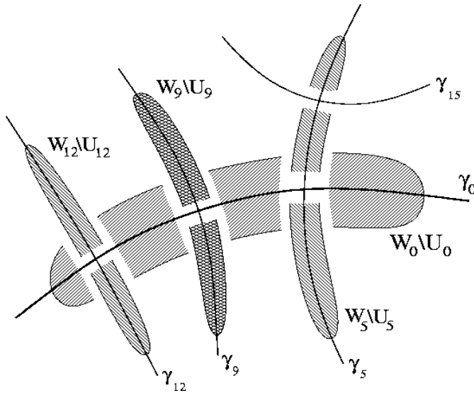
Figure 1. Avoiding self-intersections.
