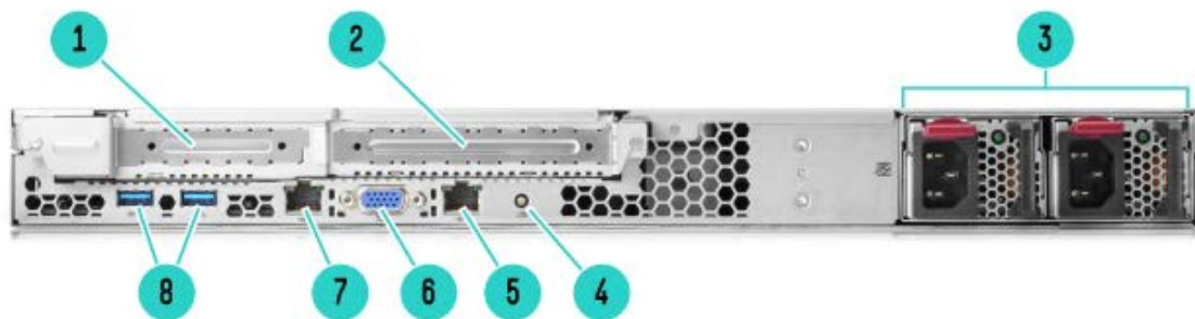
Rear View
