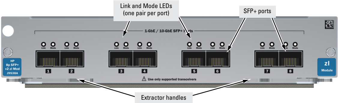
Figure 3. Example: HP 8-port 10-GbE SFP+ v2 zl Module
