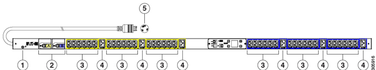
Figure 13 RP208-30M1P-6-36 PDU
