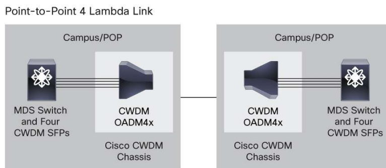
Figure 13. Point-to-Point Architecture (Dual-Fiber Link)
