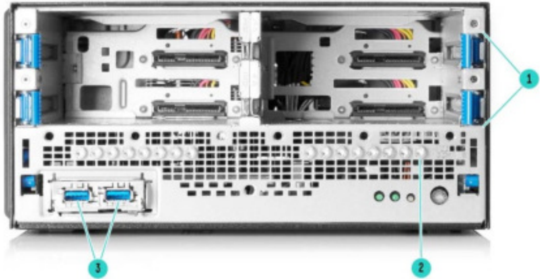
HPE ProLiant MicroServer Gen10 Plus Front View (Internal):
