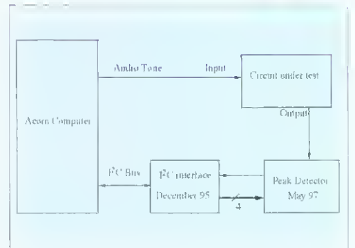
Figure 1: The Frequency Response plotter set up
