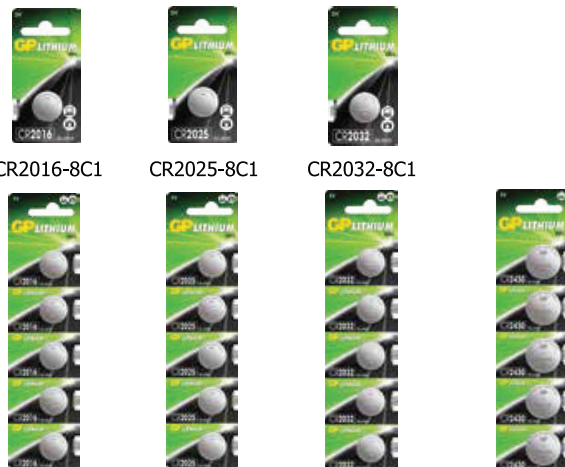
CR2016-8C1 CR2025-8C1 CR2032-8C1 CR2016TH-8C5 CR2025TH-8C5 CR2032TH-8C5 CR2430TH-8C5
