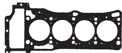
JA-01241 [QG16]
