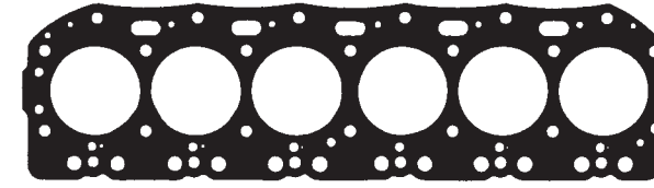
JA-11069 [2H]
