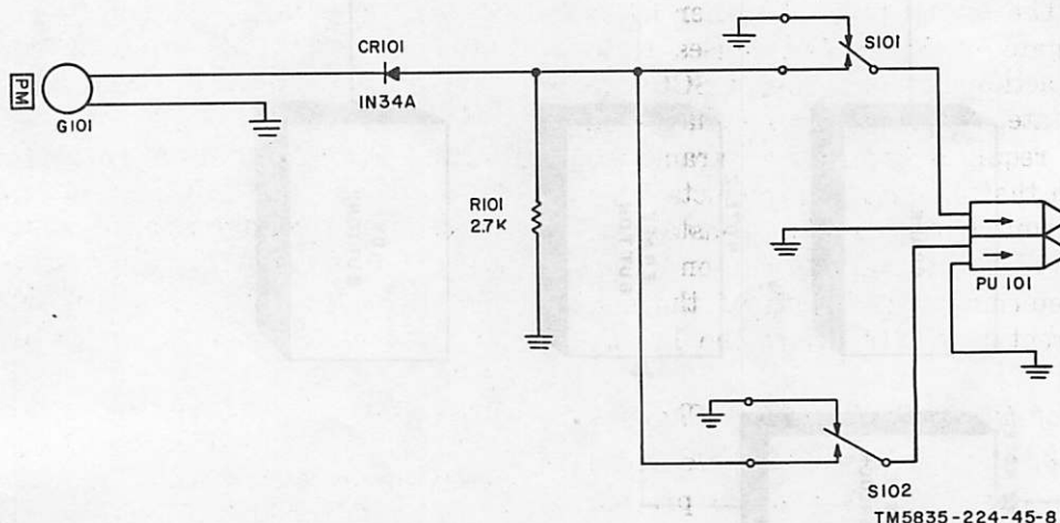
Figure 1-6. CO/B-8 coder, schematic diagram.
