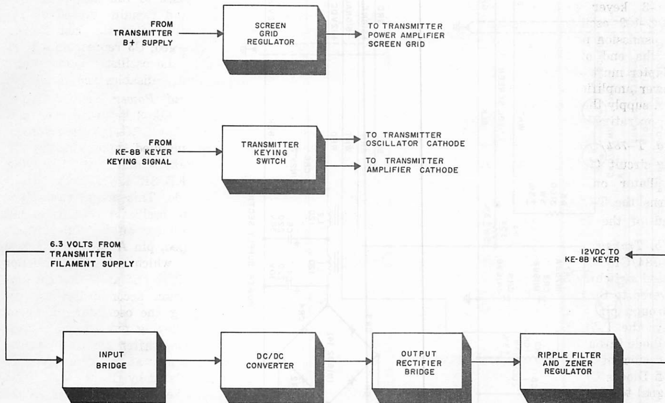
Figure 1-8. KA-3 keyer adapter, block diagram (electrical).
