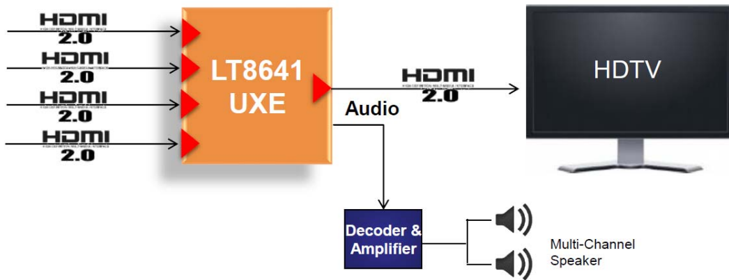
Figure 3.1 Application Diagram
