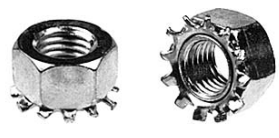
5/16-24 1/2 AF .59 OD .31 OAH GF, 34662-S, 271187
