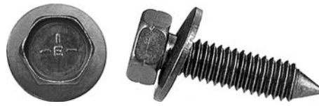
5/16-18 x 1 3/16 1/2 AF .75 CONICAL KRO, 3847962, 3992648 (sim)
