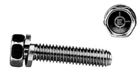
5/16-18 x 1 1/2 1/2 AF .55 SPLIT NP, 57637-S, 378335-S, 9409099
