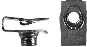
5/16-18 .16 - .22 P .67 W x 1.03 L KNR
