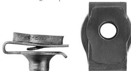
5/16-18 .02 - .13 P .88 W x 1.14 L TO, 378960-S (sim)
