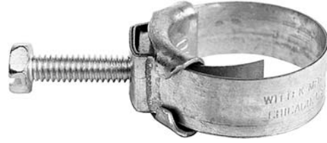
1 1/16 SIZE 1.12 MAX ID OPEN .81 CLOSED OZ, 97356-S, 9411984, 9423574 (sim), 9423575 (sim)
