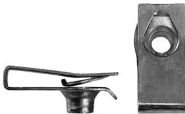
1/4-20 .02 - .15 P .58 W x 1.20 L KVG, 45267-S
