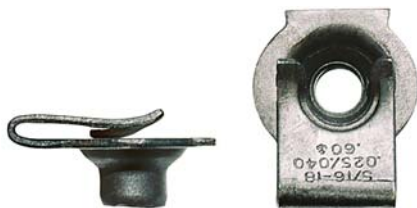
5/16-18 .02 - .06 P .88 W x 1.08 L NW
