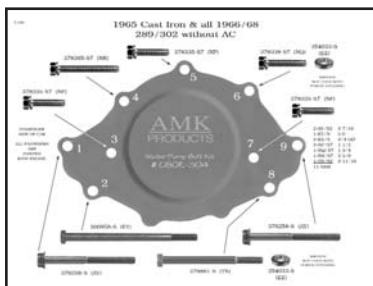
Water Pump Bolt Instructions
