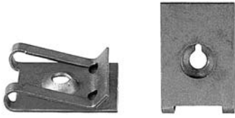
#8 .02 - .13 P .54 x .82 L EO, 45257-S, 9431530 (sim)
