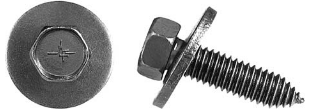
3/8-16 x 1 1/2 9/16 AF 1.12 CONICAL KJK, 407217, 10008000 (s3)
