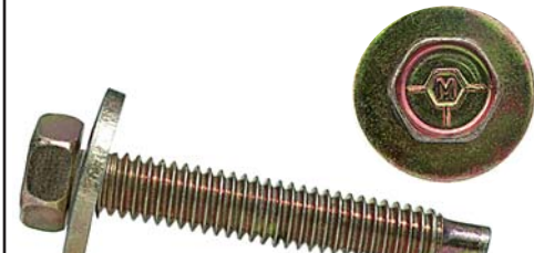
5/16-18 x 2.0 1/2 AF .88 CONICAL LWR, 57044-S
