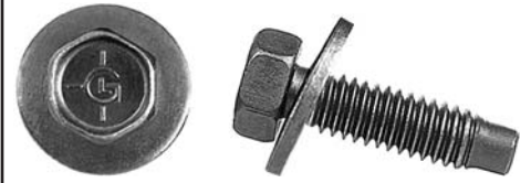
5/16-18 x 1 3/16 1/2 AF .81 CONICAL OSB, 378242-S, 378337-S (sim)
