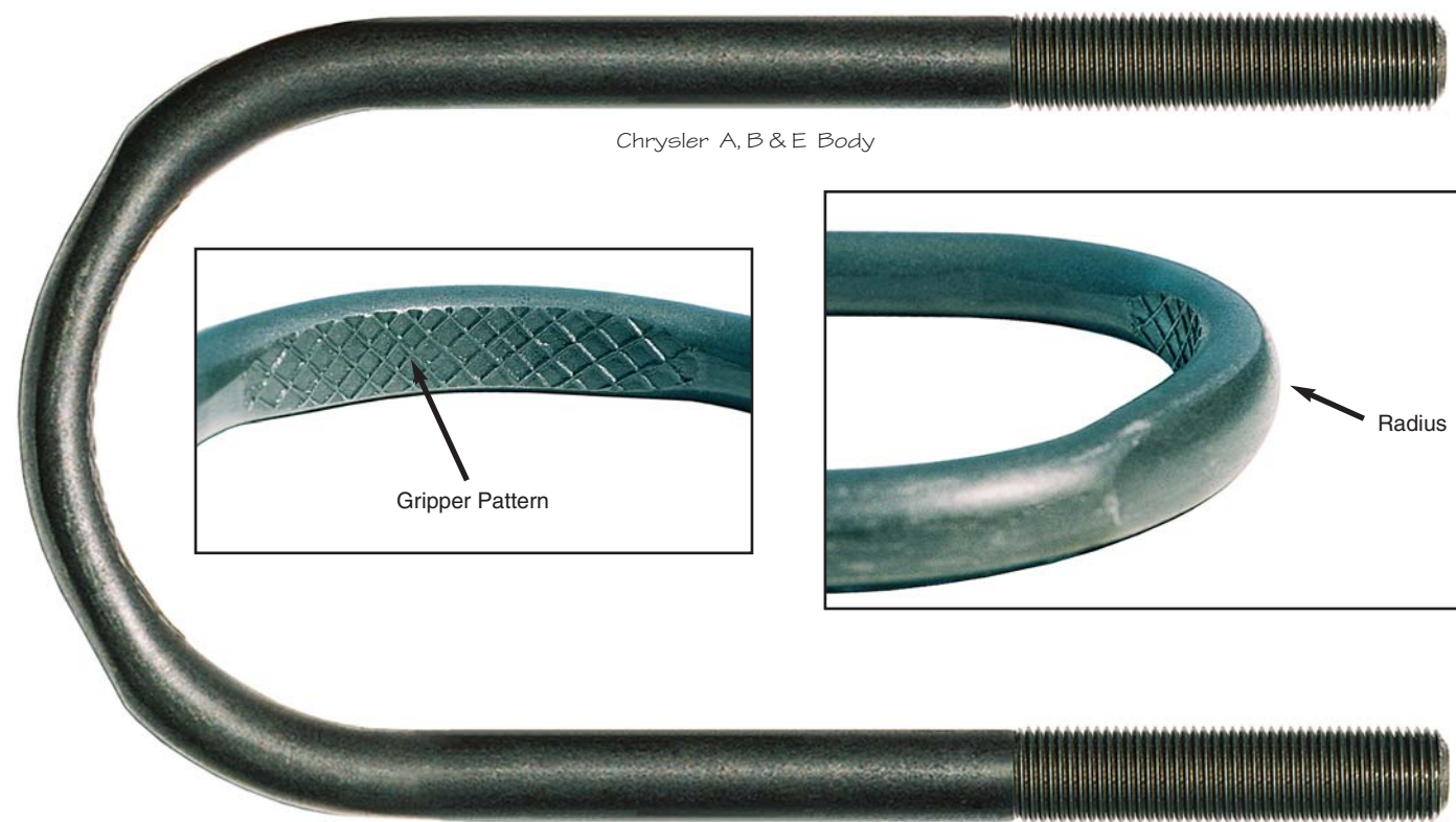
GR-5 1/2-20 x 6 5/8 3.56 C-C ONE, 1489746
