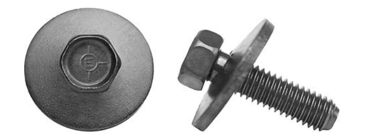
3/8-16 x 1 3/8 9/16 AF 1.31 CONICAL KQR, 3839741, 3986563 (sim)
