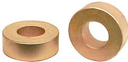
.49 ID x .35 TK x 1.0 OD OGV, 4708494 GOLD ANODIZED ALUMINUM
