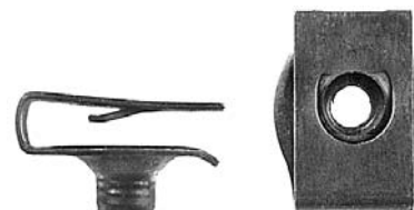
1/4-20 .14 - .20 P .74 W x .95 L KND
