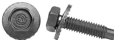
5/16-18 x 1 1/4 1/2 AF .81 TOOTHED KHW, 378242-S
