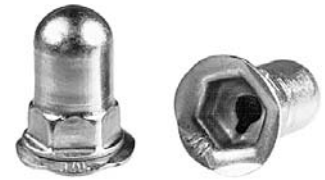
10-24 7/16 AF .63 OD .79 OAH KQG
