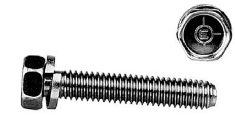
5/16-18 x 1 3/4 1/2 AF .55 SPLIT NQ, 57638-S, 378338-S, 9413364
