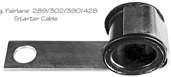
.70 CAPACITY .75 W x 3.20 L .40 HOLE OMA PLASTIC GROMMET
