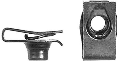
5/16-18 .02 - .15 P .66 W x 1.0 L KO, 153294 ◆, 45264-S, 1494253
