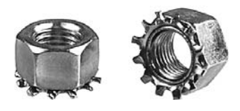
3/8-24 9/16 AF .66 OD .39 OAH JI, 34664-S, 271193 (s8)
