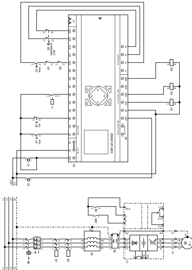
Circuit example: Two-channel Emergency-stop monitoring with easySafety
