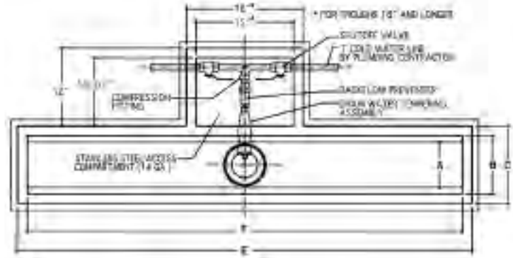
(see chart below for dimensions A through F)
