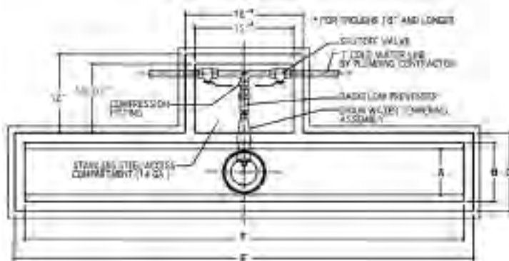
(see chart below for dimensions A through F)
