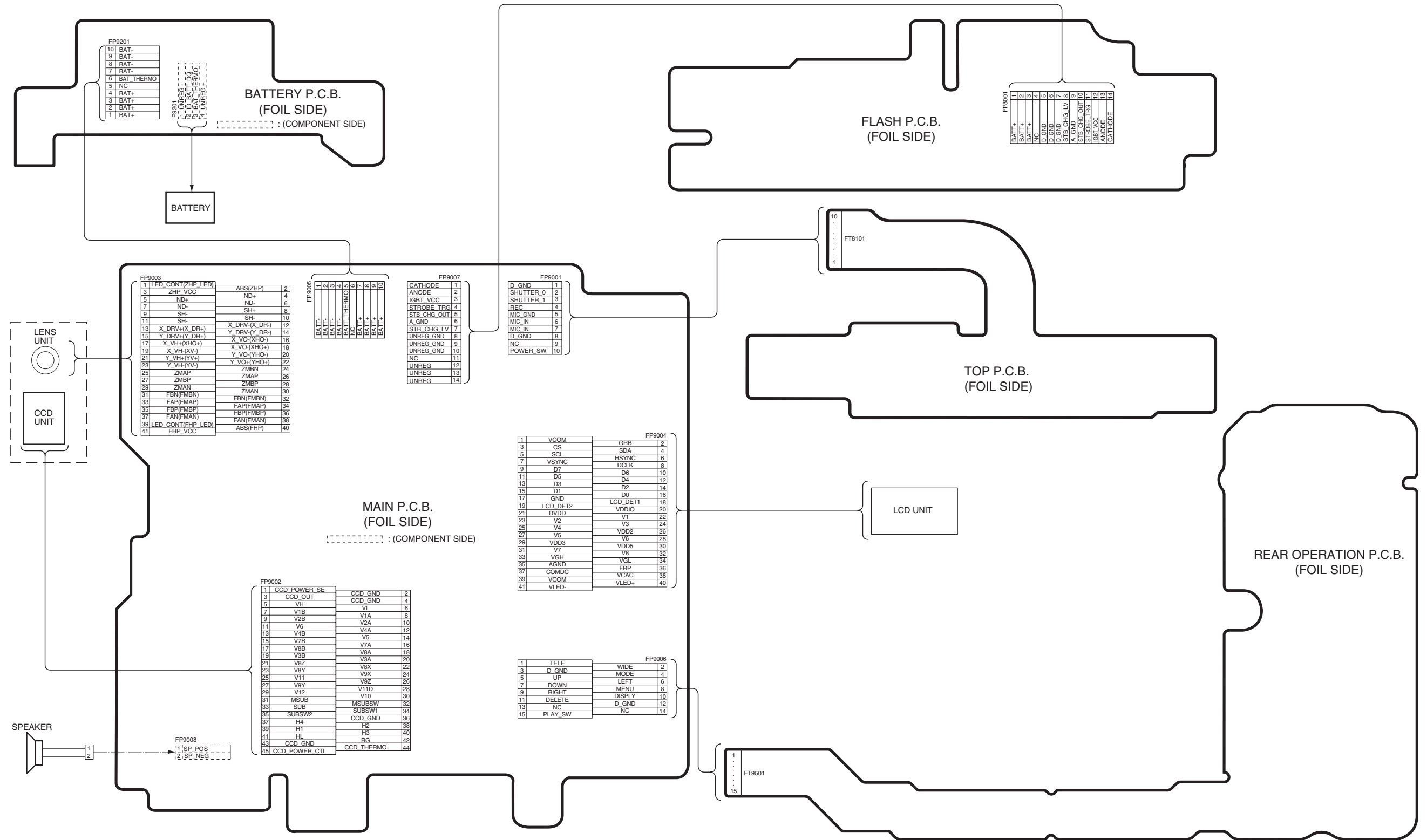
DMC-FT20/TS20 INTERCONNECTION SCHEMATIC DIAGRAM
