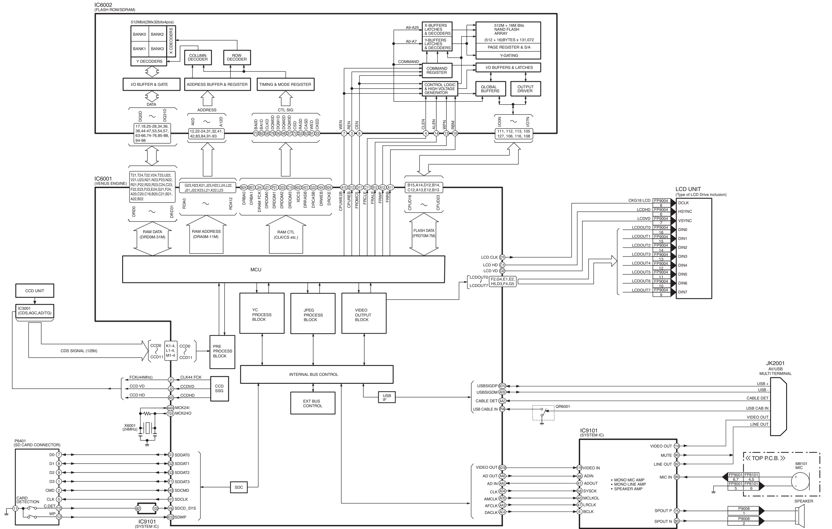
DMC-FT20/TS20 VIDEO/AUDIO PROCESS BLOCK DAIGRAM
