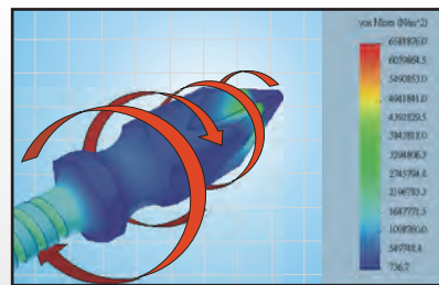
PROJAHN TORSION-Bit
