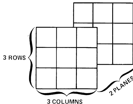
Figure 4-1 Array Representation
