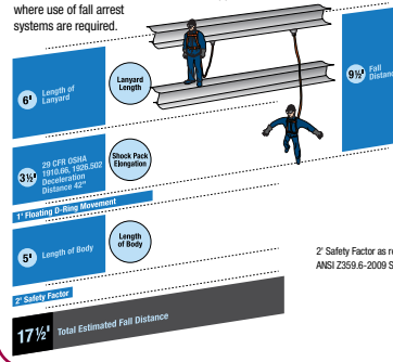
Figure B 3570 SafeStretch Lanyard
