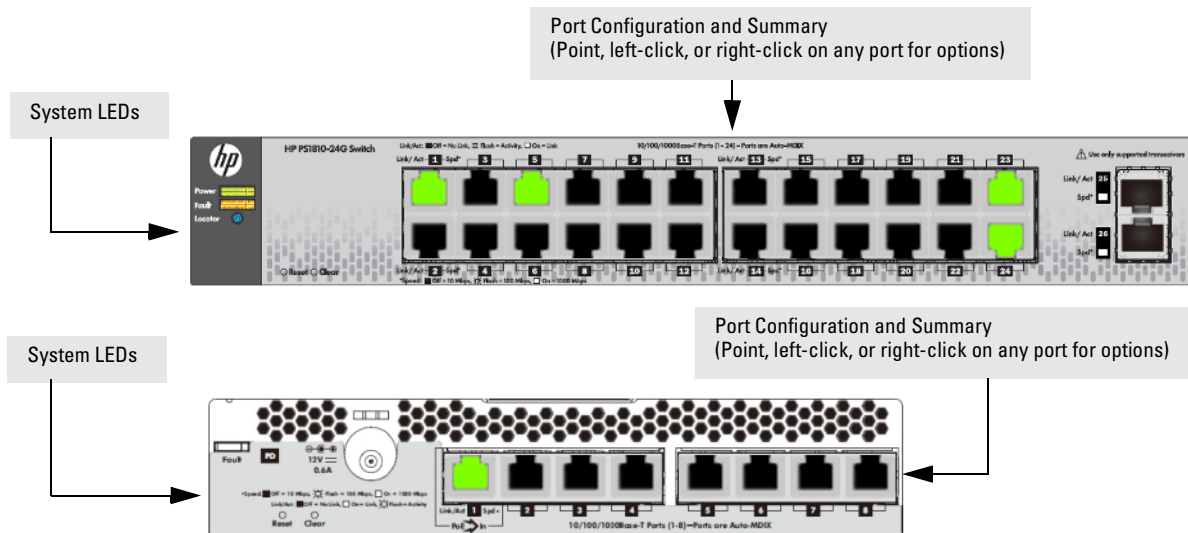
Figure 1-3. Web Applet
