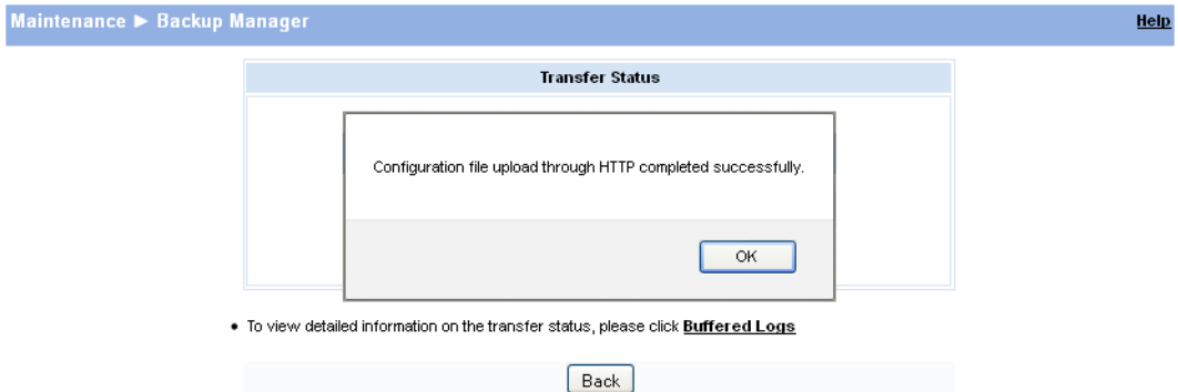
Figure 10-4. Backup Confirmation
