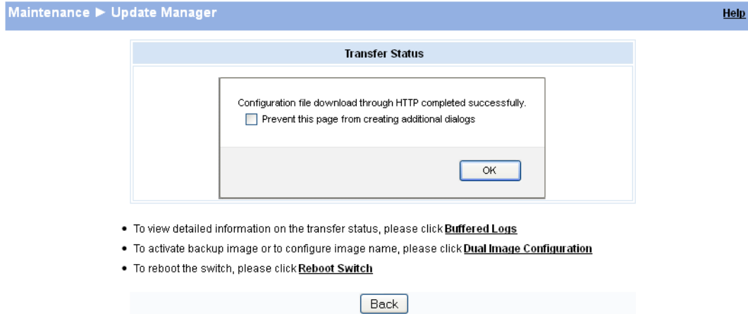
Figure 10-11. Update Confirmation
