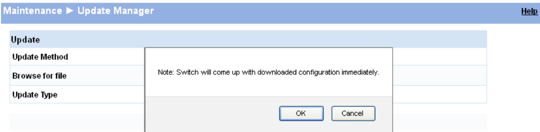
Figure 10-10. Reboot Confirmation
