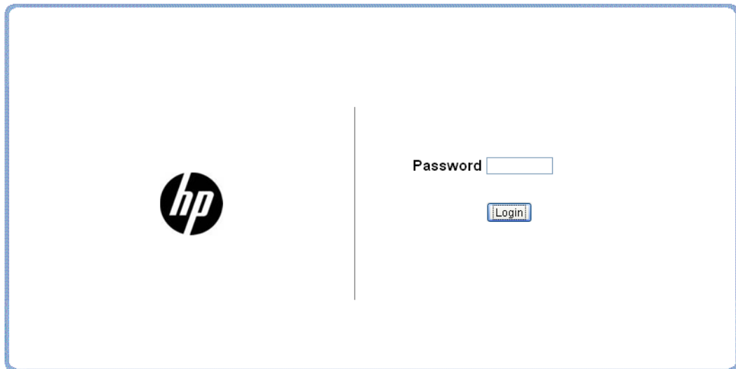
Figure 1-1. Login Page
