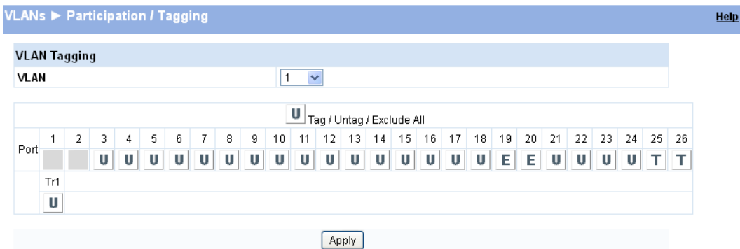
Figure 7-3. Participation/Tagging Page
