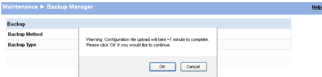
Figure 10-2. Backup Warning
