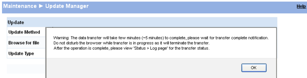
Figure 10-7. Update Warning
