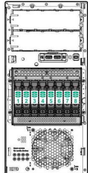
1-8 8 x SFF SAS/SATA/SSD hot pluggable hard drive bays
