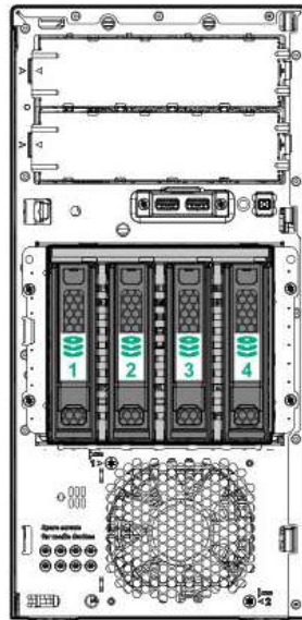
1-4 4 x LFF SAS/SATA/SSD hot pluggable hard drive bays
