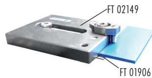
FT 02149 F-Tool universal clamping beam supporting plate in the single application
