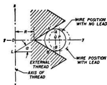
FIGURE 13.1.—Basis of lead angle correction for external thread.
