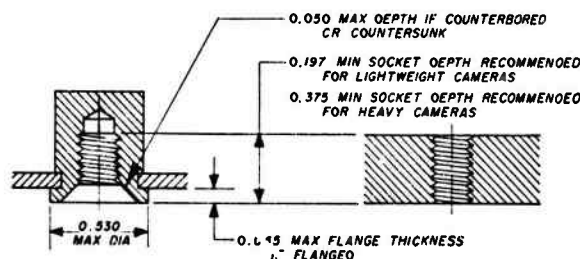
FIGURE XVIII.2.—Tripod socket in camera, \frac{1}{4} -20 UNC-1B.
